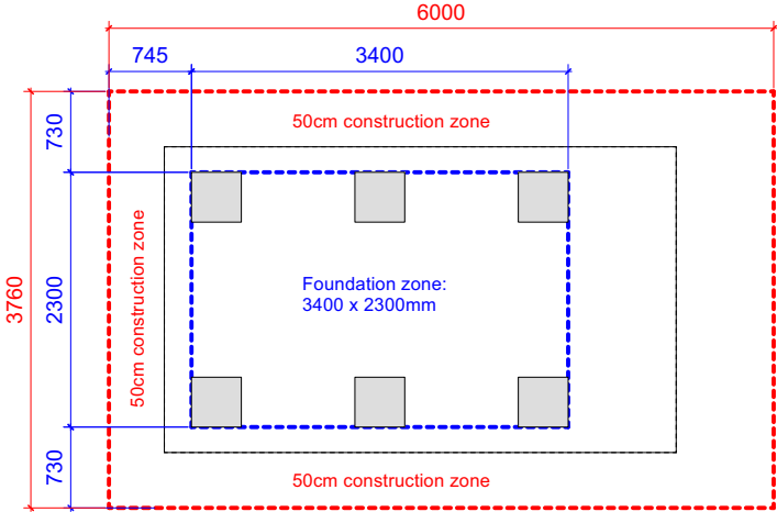
Mökki Shelter foundation area
