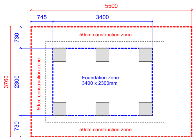
Mökki Tube Long foundation area
