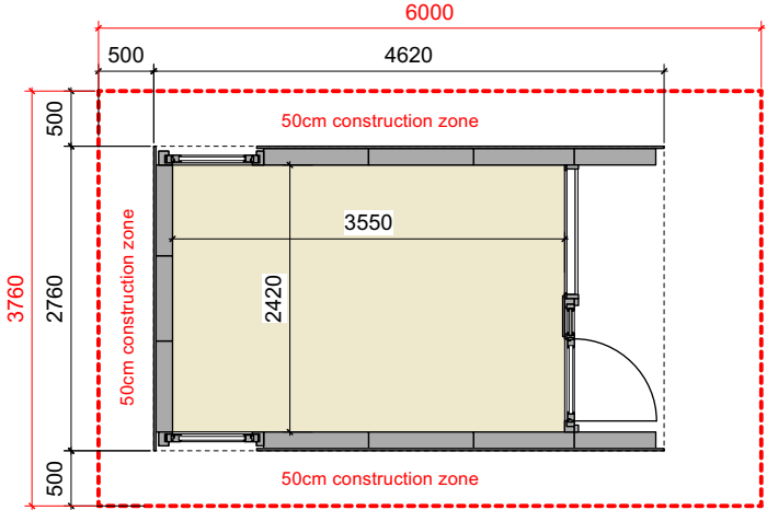
Mökki Shelter space required
