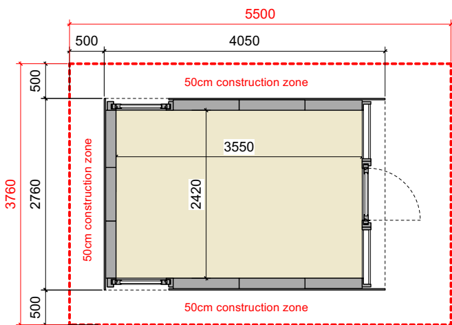
Mökki Tube Long space required
