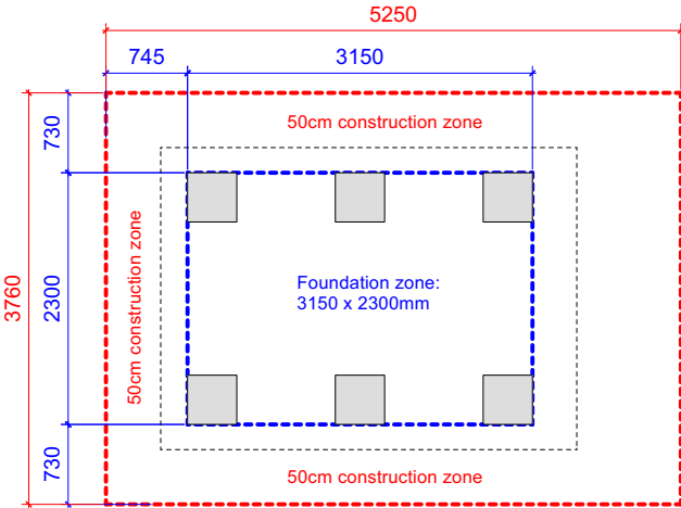
Mökki Tube Compact foundation area
