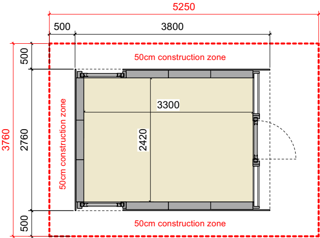
Mökki Tube Compact space required
